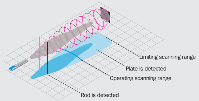
Every ultrasonic sensor has its characteristic club-shaped detection range. It is narrow for smaller objects and wide for larger ones. The typical detection areas are depicted by sound-beam diagrams.
