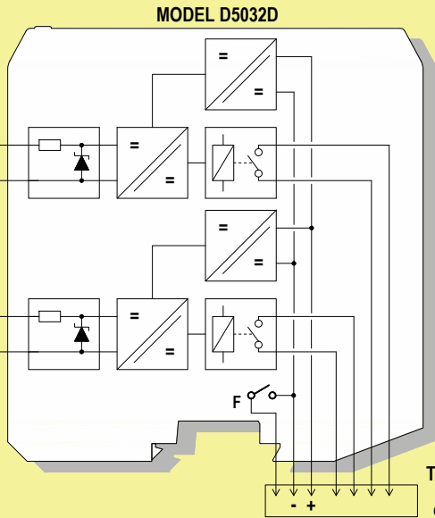
MODEL D5032D Duplicator or Fault Out
