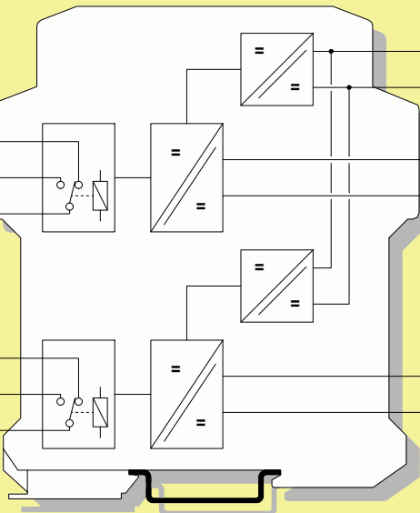
MODEL D1044D Loop powered (1oo2 channel architecture)
