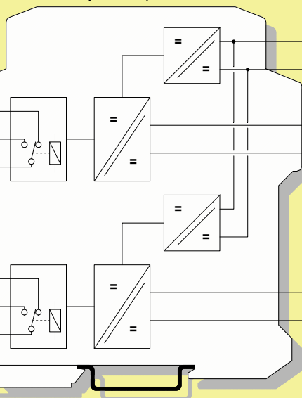
MODEL D1044D Bus powered (1oo2 channel architecture)
