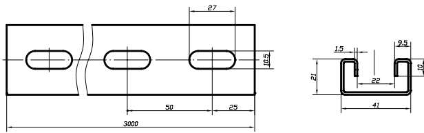
"U" Section 41x21
