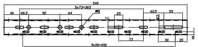
Bracket base for mesh tray
