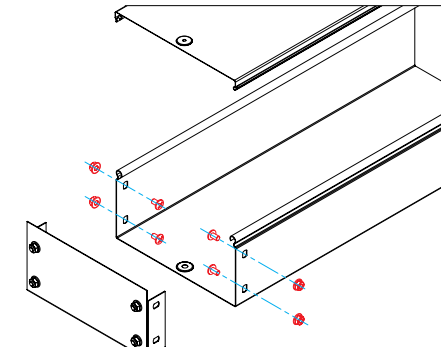
End cap h 50/100 mm
