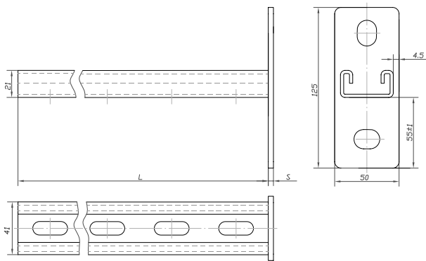
MP Cantilever "C" profile 41x21
