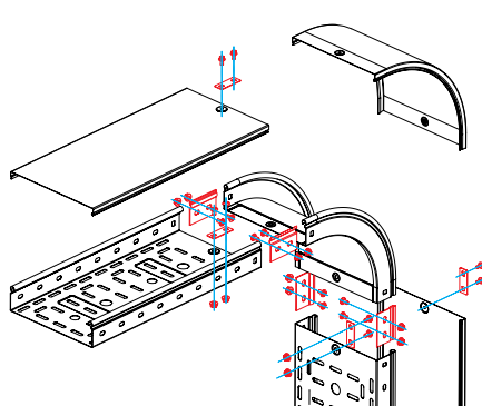
Falling elbow 90°
