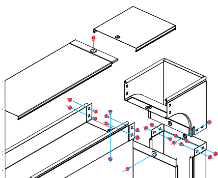
Falling elbow with plane inversion
