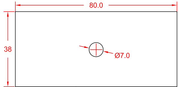
Junction plate with hole
