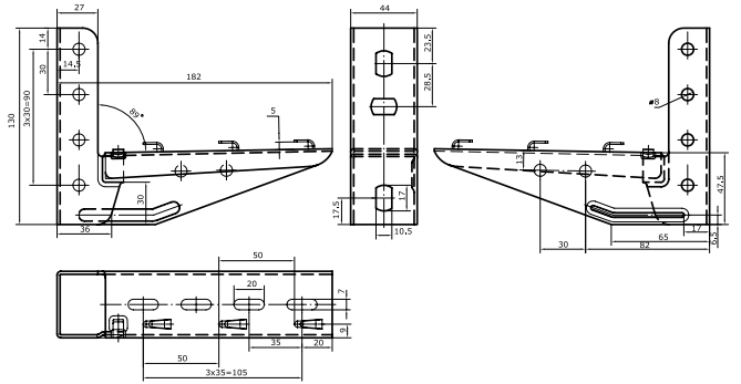
Bracket for mesh tray
