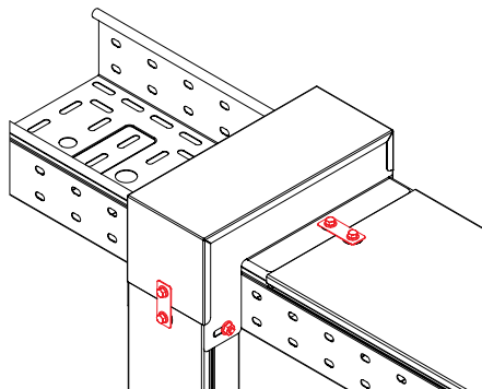
Vertical falling elbow as cover
