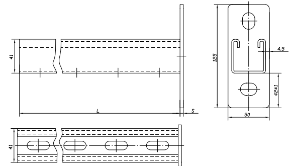
MP Cantilever "C" profile 41x41
