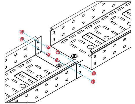
"Female" and "male" ends - h 100 mm
