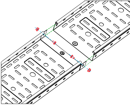
"Female" and "male" ends - h 50 mm
