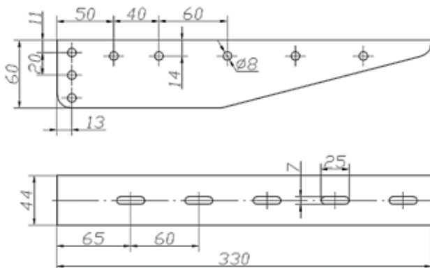
Bracket base
