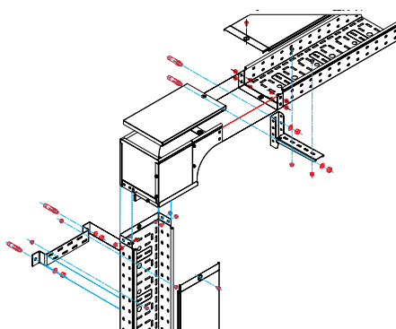
Skew right falling elbow 90°
