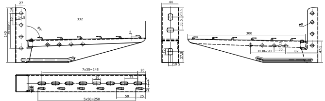
Bracket for mesh tray
