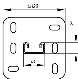
Single Vertical support "C" profile
