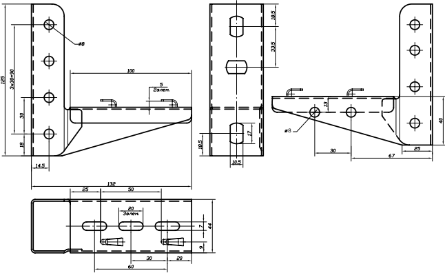
Bracket for mesh tray
