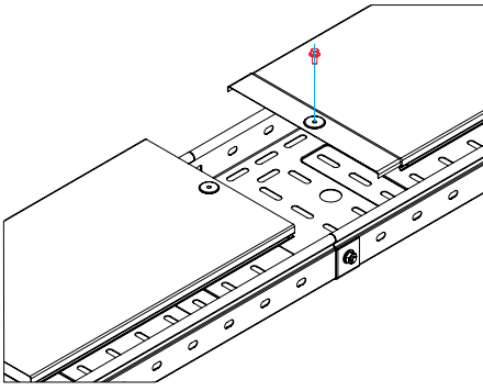
Covers snap onto the base straight elements.
