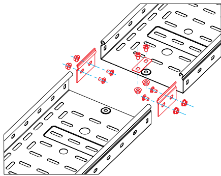
Joint plate - h 50 mm
