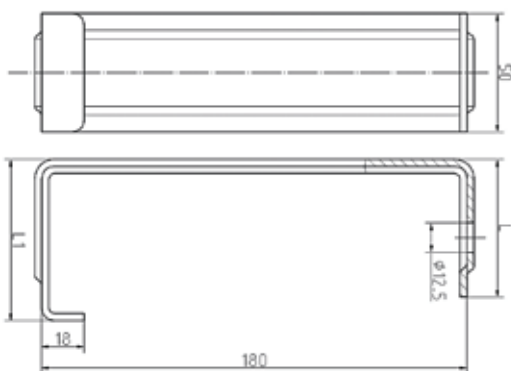
C-bracket
