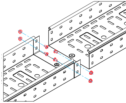
"Female" and "male" ends - h 80 mm.
