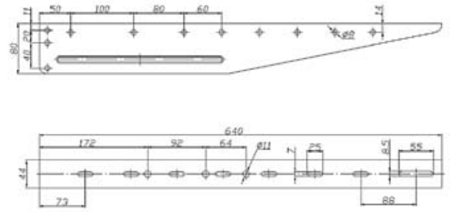
Bracket base
