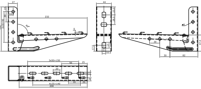
Bracket for mesh tray
