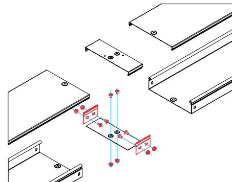
Joint for base and joint for cover
