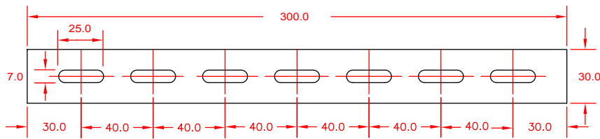
Side-joint plate
