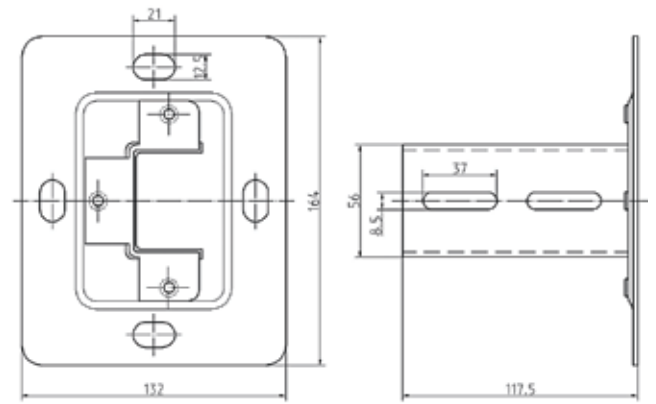
SSM Ceiling support
