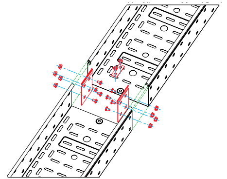
Joint plate - h 100 mm
