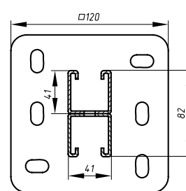
Double Vertical support "C" profile
