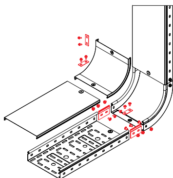
Rising elbow 90°
