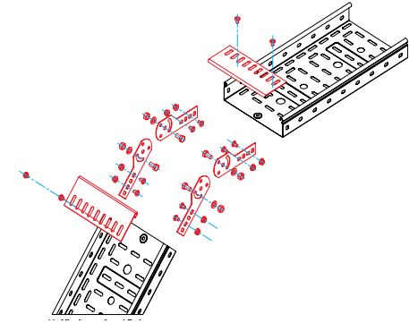
protective plate and articulated vertical joint
