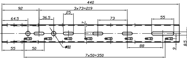
Bracket base for mesh tray
