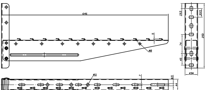
Bracket with rivets for mesh tray
