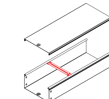
Cable Holder
