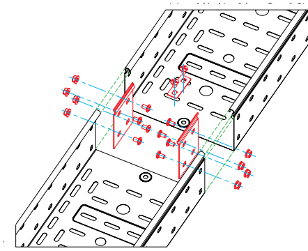
Joint plate- h 80 mm
