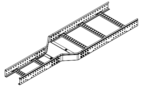
Cable Ladders L5 Combitech fully compatible with accessories of C5 Combitech system
