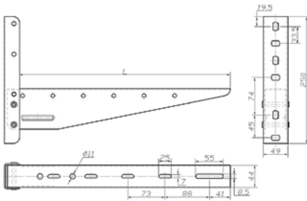
Bracket with rivets
