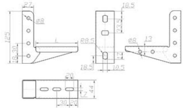
Bracket
