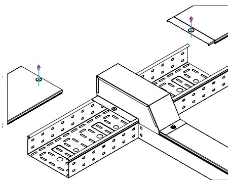
Horizontal tee as cover
