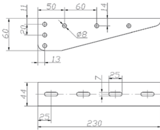
Bracket base
