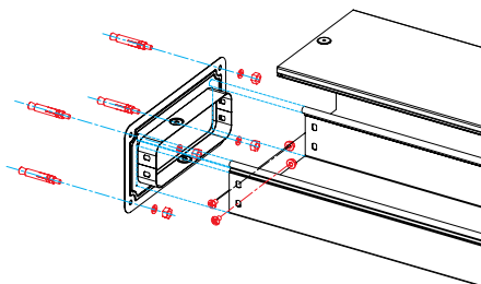
Connection flange
