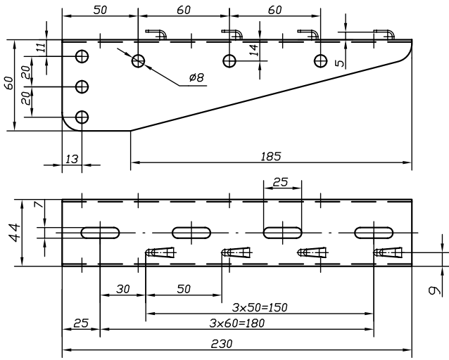
Bracket base for mesh tray
