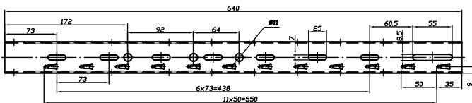
Bracket base for mesh tray
