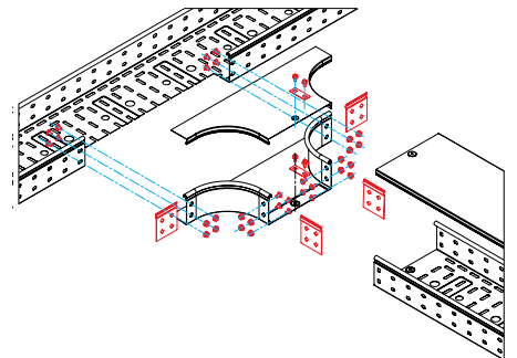
Lateral horizontal tee
