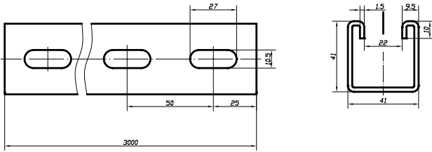
"U" Section 41x41
