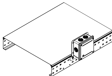
Vertical Mounting Plate
