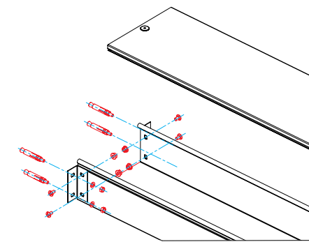
Wall mounting
