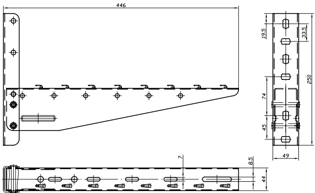
Bracket with rivets for mesh tray
