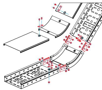
Rising elbow 45°
