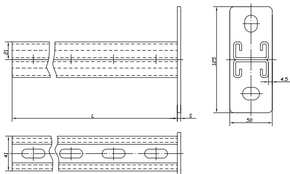
MP Cantilever "C" double profile 41x21
