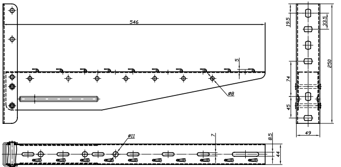
Bracket with rivets for mesh tray
