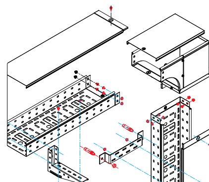
Skew left falling elbow 90°
