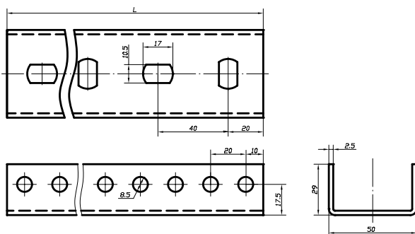
U-Section
