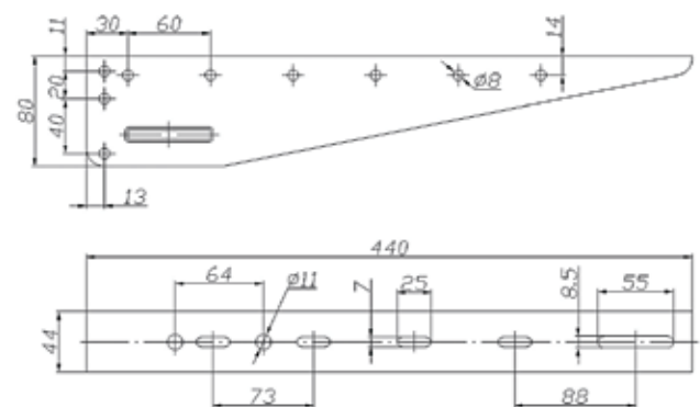
Bracket base
