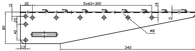
Bracket base for mesh tray
