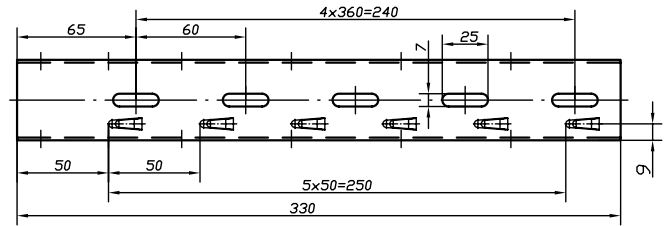
Bracket base for mesh tray
